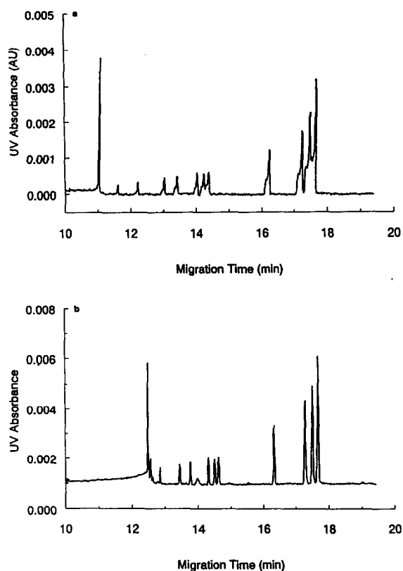
Fig. 2. (a) Electropherogram of a 50 \mu g/ml \Phi X-174 RF DNA HaeIII dissolved in 20 mM NaCl. Conditions and peak assignments as in Fig. 1a. (b) Influence of presample injection of 0.1 M Tris–acetate pH 8.3. Injection procedure: first injection: 10-s pressure injection of Tris–acetate; second injection: 20-s pressure injection of 50 \mu g/ml \Phi X-174 HaeIII sample in 20 mM NaCl.
