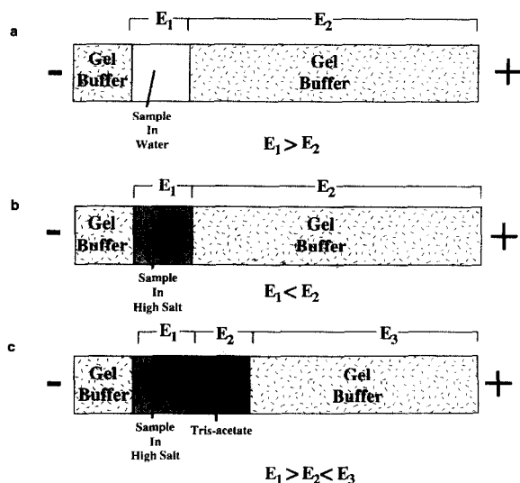
Fig. 3. Axial electric field profiles for (a) injection of sample in water, (b) injection of sample in high salt and (c) double injection technique as described in text.
