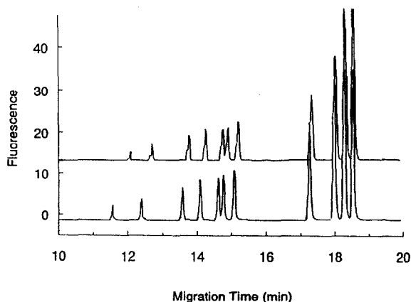
Fig. 4. High ionic strength samples cause a migration time shift. Upper electropherogram: 50 \mu\text{g/ml} \Phi\text{X-174} HaeIII in 20 mM NaCl. Lower electropherogram: 50 \mu\text{g/ml} \Phi\text{X-174} HaeIII in water. Conditions and peak assignments as in Fig. 1a; detection: LIF.
