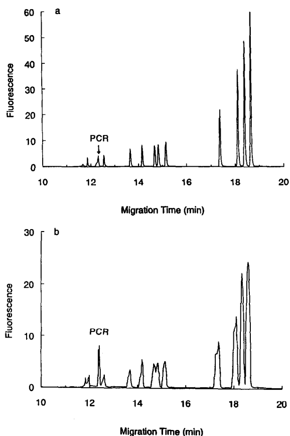
Fig. 5. (a) Electropherogram of PCR sample and DNA standard. First injection: PCR sample (Sabin 3, 97 bp); second injection: \Phi X-174 HaeIII 10 \mu g/ml. (b) Electropherogram of DNA standard and PCR sample. First injection: \Phi X-174 HaeIII 10 \mu g/ml; second injection: PCR sample (Sabin 3, 97 bp). Peak assignment and conditions as in Fig. 4; PCR = peak of PCR product.
